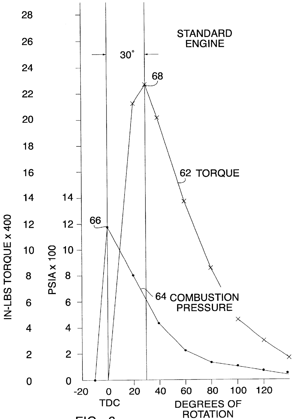
FIG. 6 PRIOR ART
